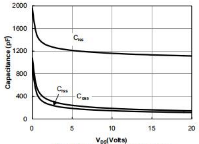
Figure 8: Capacitance Characteristics
