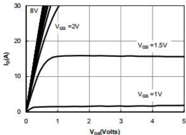
Figure 1: On-Regions Characteristics
